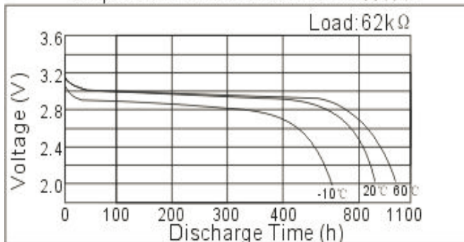
Temperature Characteristics / 温度特性
