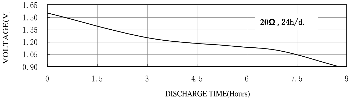
Typical Discharge Characteristics at 20°C
