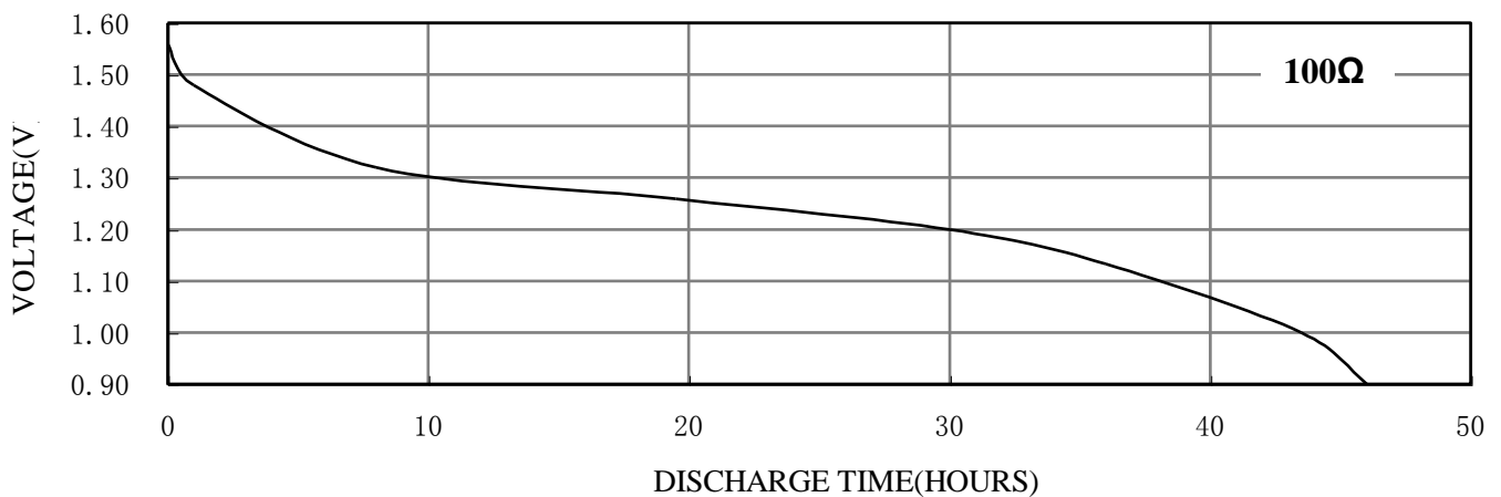
Typical Discharge Characteristics at 20°C
